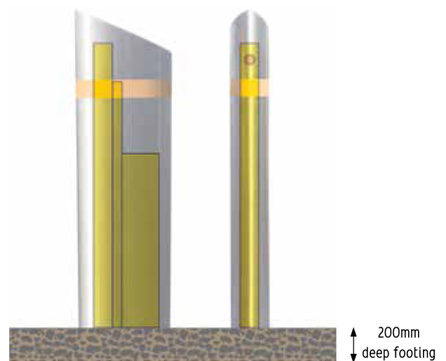
Spring Bollard Cover Side View
